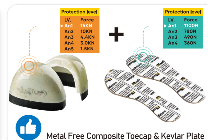
Slip Resistant & Abrasion Resistant & Heat Resistant
