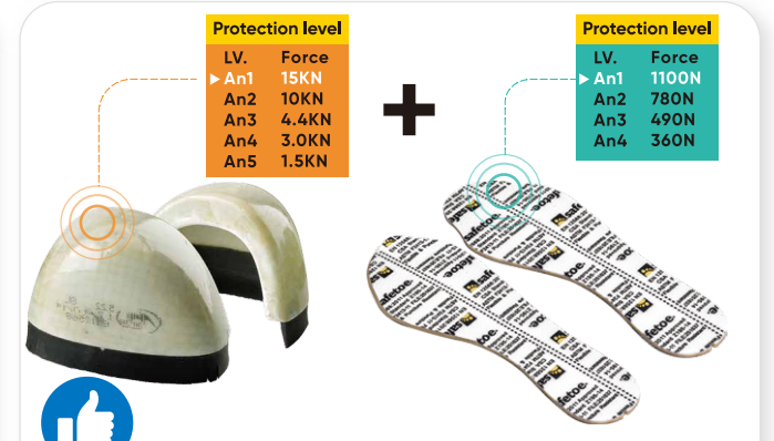
Metal Free Composite Toecap & Kevlar Plate
