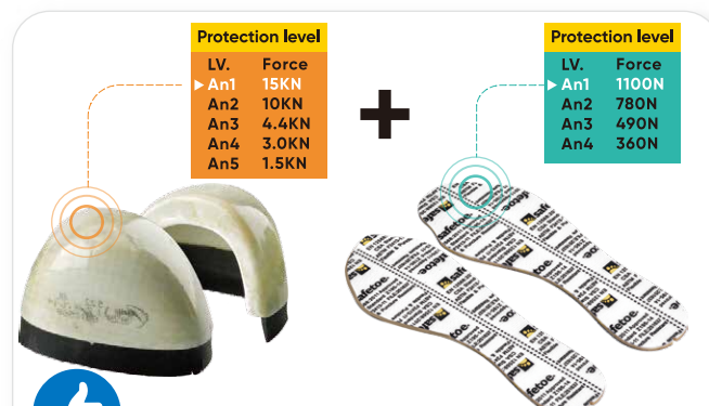
Metal Free Composite Toecap & Kevlar Plate
