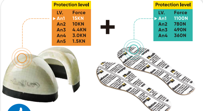
Metal Free Composite Toecap & Kevlar Plate
